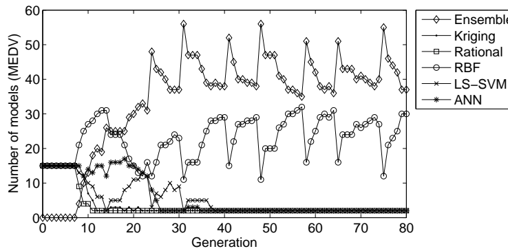
Figure 26: BH: Oscillations in the population evolution ( HGA_{EP=true} )
