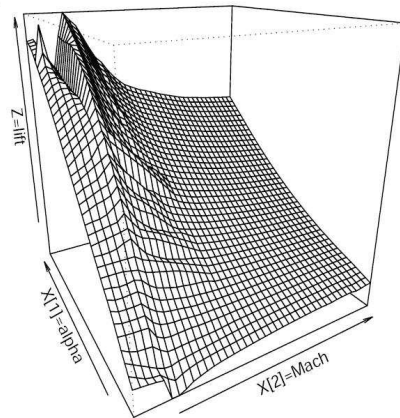
(b) Lift plotted as a function of speed and angle of attack with side-slip angle fixed to zero (Gramacy et al., 2004).
