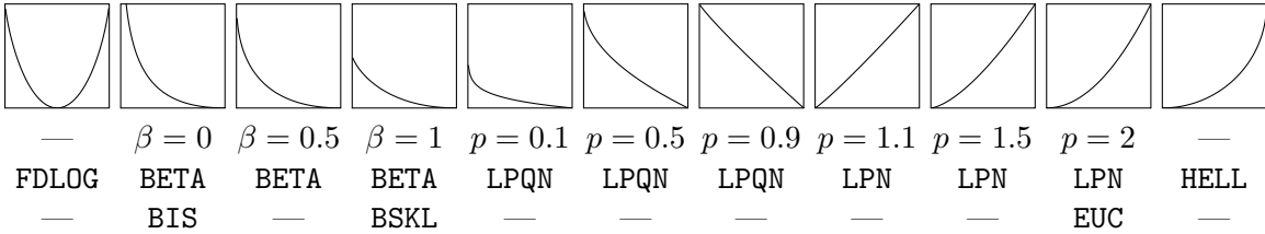
Figure 2: Separable regularizers on (0, 1) .
