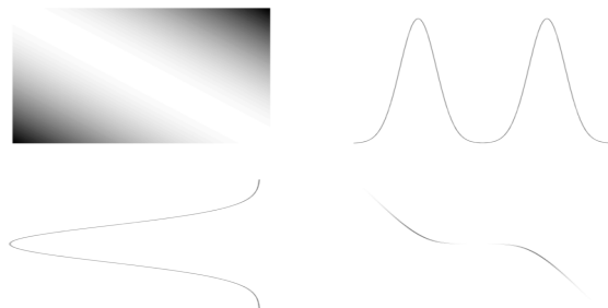
Figure 3: Earth mover’s plan \pi^* for the cost matrix \gamma and input distributions \mathbf{p}, \mathbf{q} .
