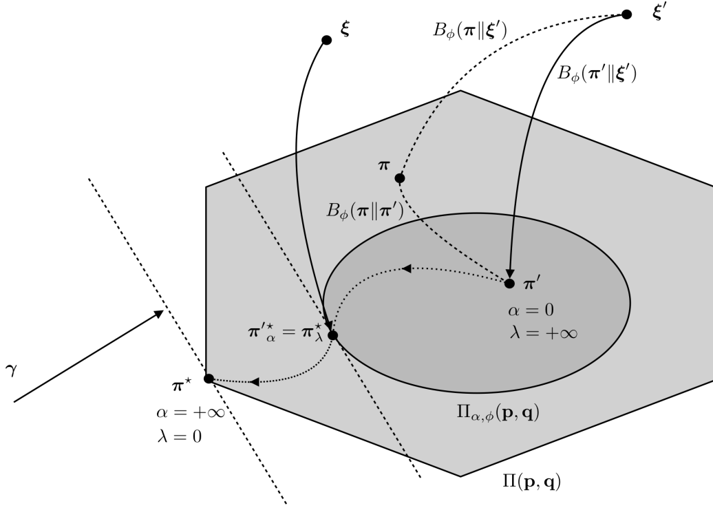
Figure 1: Geometry of regularized optimal transport.
