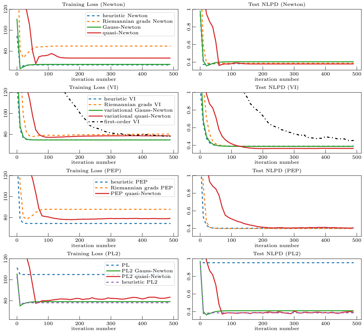
Figure 3: Heteroscedastic noise results. Mean of 4-fold cross validation shown. Variational quasi-Newton is capable of obtaining the best predictive performance, however all quasi-Newton methods converge slowly due to the need for damping. Gauss–Newton variants obtain similar performance to the heuristic method, but do not require computation of second-order derivatives. PL2 is the second-order PL method, and it significantly outperforms PL because it takes into account the gradients of the likelihood covariance.
