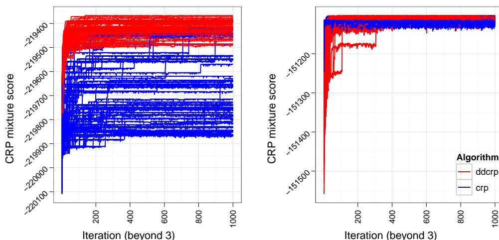
Figure 7: Each panel illustrates 100 Gibbs runs using Algorithm 3 of Neal (2000) (CRP, in blue) and the sampler from Section 3 with the identity decay function (distance dependent CRP, in red). Both samplers have the same limiting distribution because the distance dependent CRP with identity decay is the traditional CRP. We plot the log probability of the CRP representation (i.e., the divergence) as a function of its iteration. The left panel shows the Science corpus, and the right panel shows the New York Times corpus. Higher values indicate that the chain has found a better local mode of the posterior. In these examples, the distance dependent CRP Gibbs sampler mixes faster.
