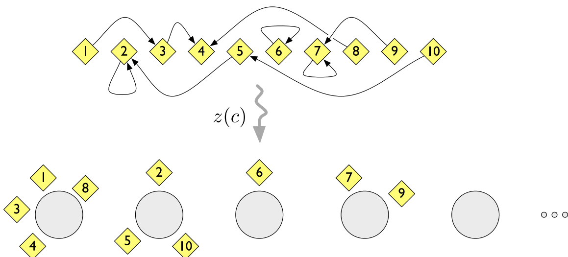
Figure 1: An illustration of the distance dependent CRP. The process operates at the level of customer assignments, where each customer chooses either another customer or no customer according to Equation (2). Customers that chose not to connect to another are indicated with a self link. The table assignments, a representation of the partition that is familiar to the CRP, are derived from the customer assignments.
