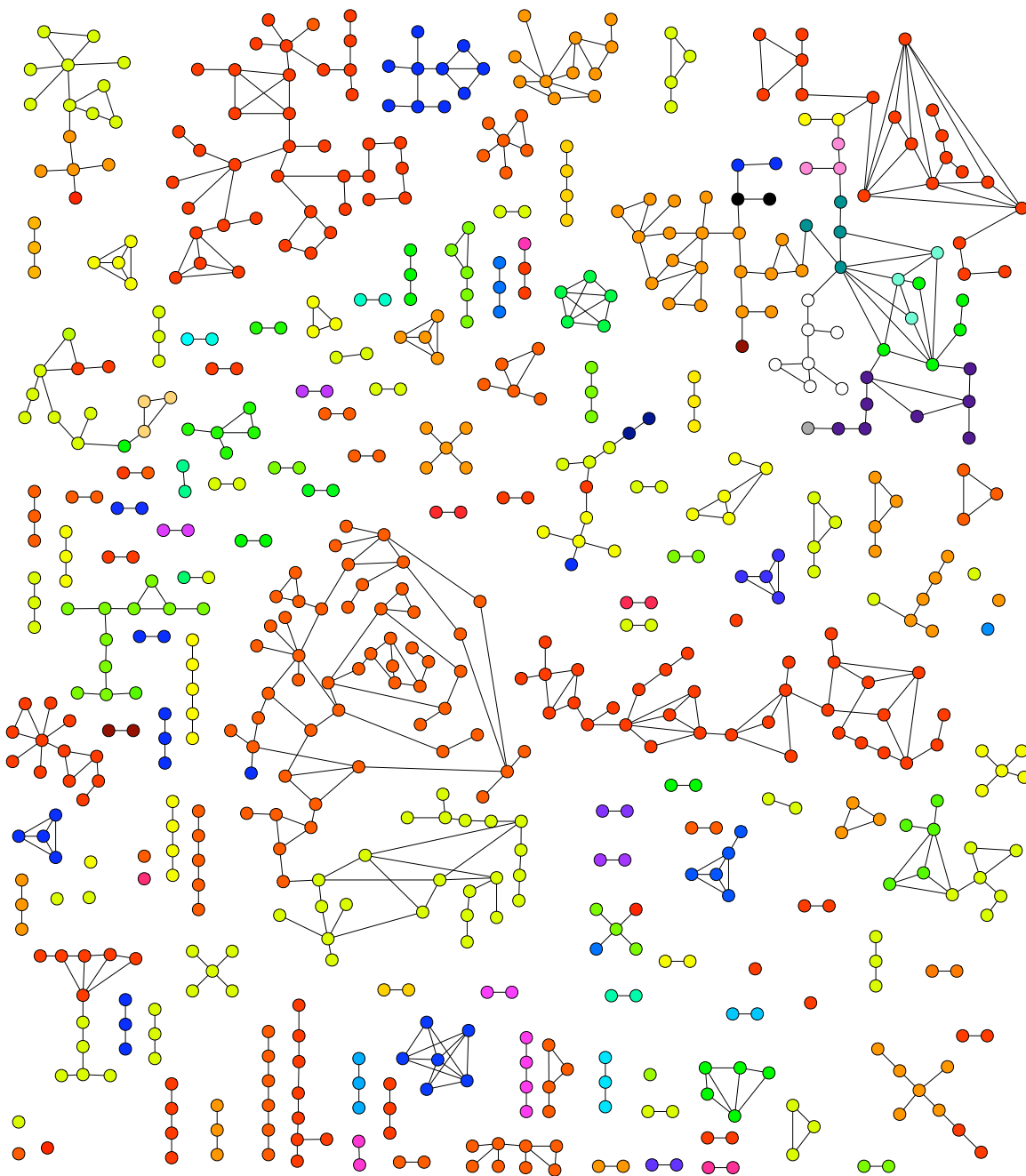
Figure 6: The MAP clustering of a subset of CORA. Each node is an abstract in the collection and each link represents a citation. Colors are repeated across connected components—no two data points from disconnected components in the graph can be assigned to the same cluster. Within each connected component, colors are not repeated, and nodes with the same color are assigned to the same cluster.
