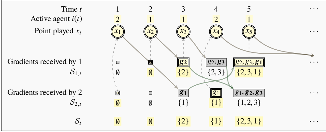
Figure 2: Illustration of the type of feedback sequences that may occur in a multi-agent setting. In the standard single-agent case, the feedback sequence \mathcal{S}_t, t = 1, 2, \dots , is necessarily non-decreasing: even though the feedback may not arrive with the same order as the corresponding actions, the number of available gradients can only grow. This no longer holds when multiple agents are involved in the optimization process.
