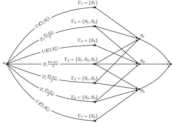
Figure 9: Minimum cost flow problem formulation for the general subset S , comprising maximal c -components S = S_1 \cup S_2 \cup S_3 . All the non-specified edges have capacity of 1 and cost of 0, i.e., \gamma \setminus \zeta = 1 \setminus 0 .
