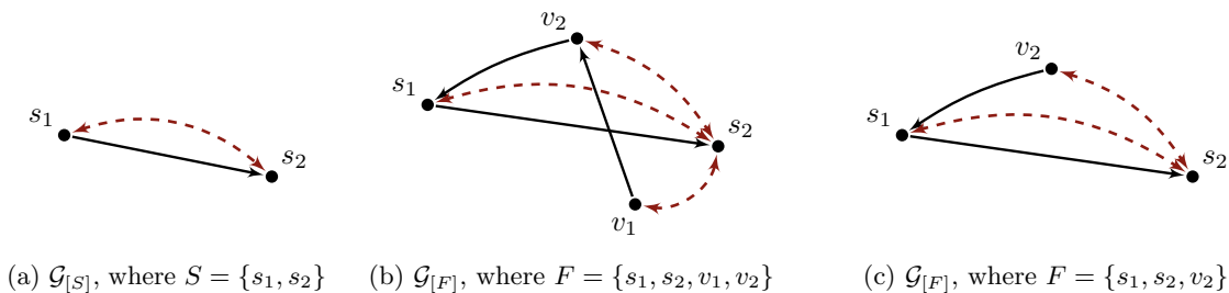
Figure 3: Two hedges formed for Q[S] in the graph of Figure 2a.
