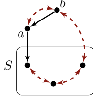
Figure 15: Hedges of size 2 must be in the form depicted above. Exactly one vertex a is a member of \mathbf{pa}(S) \setminus \mathbf{biD}(S) , and the other vertex b is a member of \mathbf{biD}(S) \setminus \mathbf{pa}(S) .
