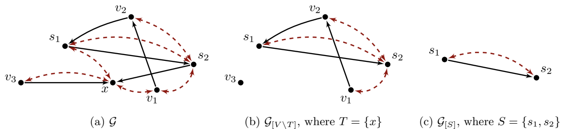
Figure 2: An example of reformulating an arbitrary causal query in the form of Q[\cdot] . P(S|do(T)) is identifiable if and only if Q[\mathbf{Anc}_{\mathcal{G} \setminus T}(S)] is identifiable. Given S = \{s_1, s_2\} and T = \{x\} , from Fig. 2b, it is evident that \mathbf{Anc}_{\mathcal{G} \setminus T}(S) = \{v_1, v_2, s_1, s_2\} .
