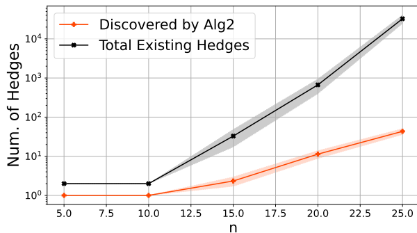
Figure 11: Number of the total hedges formed for Q[S] vs the number of hedges Algorithm 2 discovers until finding the optimal solution.
