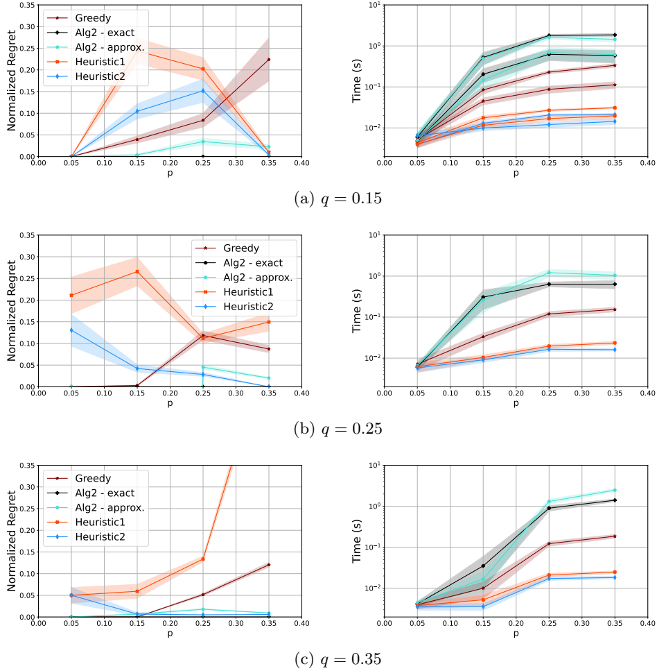
Figure 19: The effect of the density of directed edges. Random graphs of size n = 30 are generated with different densities of bidirected edges.
