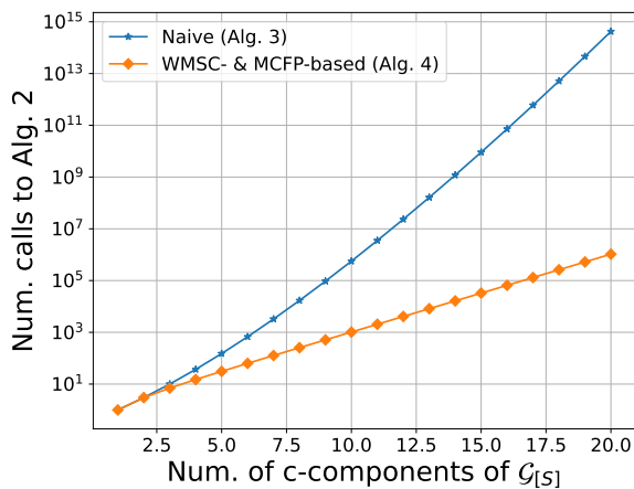
Figure 12: Number of calls to Algorithm 2 as subroutine, vs the number of c-components of \mathcal{G}_{[S]} .
