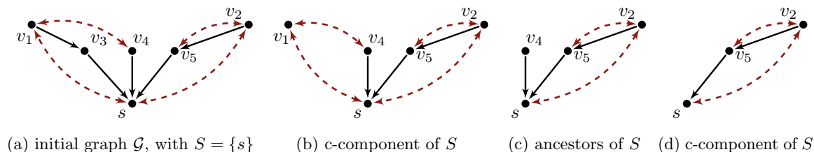
Figure 6: An example showing how Algorithm 1 works, alternating between keeping only the c-component of S , and then keeping only the ancestors of S in the remaining graph.
