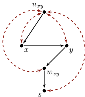
Figure 13: Reduction from the weighted vertex cover problem to the minimum-cost intervention problem. Each edge \{x, y\} in the undirected graph \mathcal{H} is represented by a hedge structure in the semi-Markovian graph \mathcal{G} .
