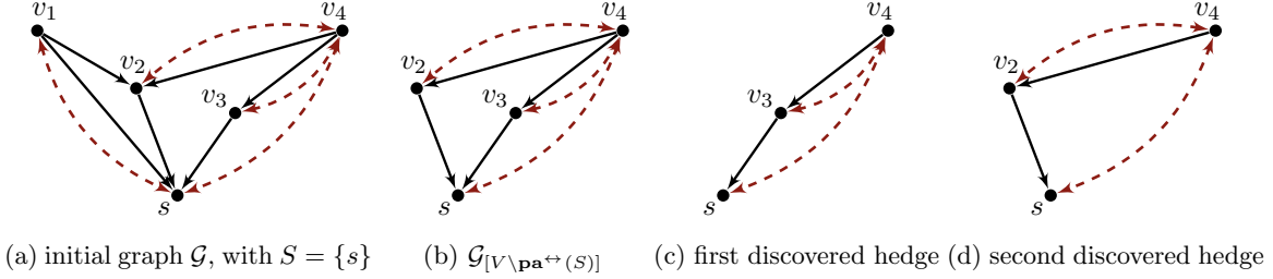
Figure 7: An example showing how Algorithm 2 works, by discovering sufficiently many hedges to circumvent the need for enumerating all of them. See also Figure 11.
