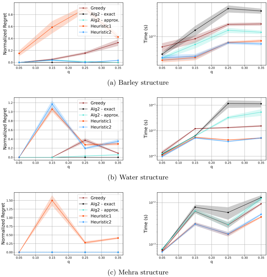
Figure 16: The performance of the proposed algorithms on three real-world structures.
