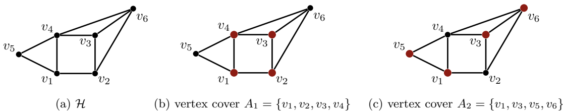
Figure 4: An example of a WMVC problem with two of its vertex covers.
