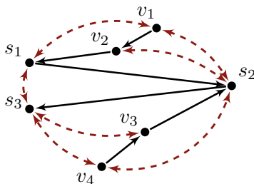
Figure 8: An example where the optimal interventions collection is not a singleton, i.e., a solution to (2) is not a solution to (1). In this example, the cost of intervening on each of \{s_1, s_2, s_3\} is 1, whereas the cost of intervening on each of \{v_1, v_2, v_3, v_4\} is 5.
