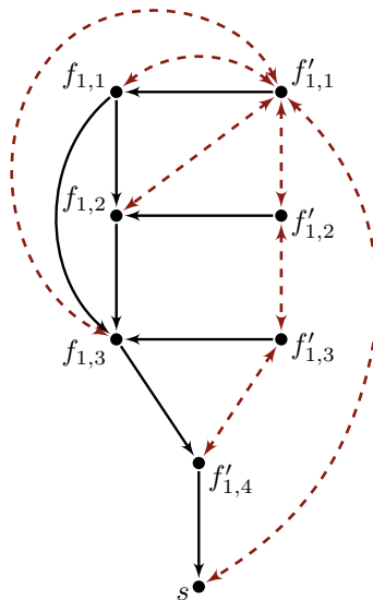
Figure 14: Reduction from the minimum weighted hitting set problem to the minimum-cost intervention problem. Each set F_i = \{f_{i,1}, \dots, f_{i,m}\} is represented by a hedge structure in the semi-Markovian graph \mathcal{G} .
