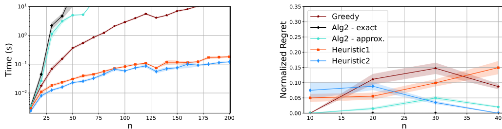
Figure 10: Evaluation of our algorithms in terms of runtime (Left) and normalized regret (Right). n represents the number of vertices in the causal graph, Alg2-exact and Alg2-approx. solve the minimum hitting set exactly and approximately, respectively, and the greedy algorithm is presented in Appendix E. Alg2-exact obtains zero regret.
