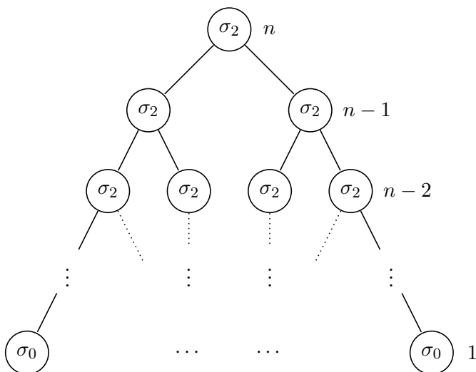
Figure 1: Tree t_n
