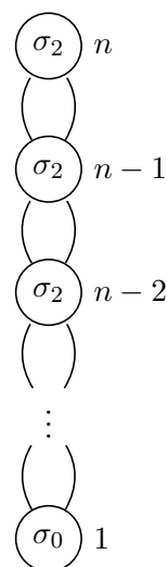
Figure 2: DAG G_n
