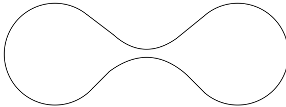
Figure 2: Curve in \mathbb{R}^2 where \tau \ll \iota .
