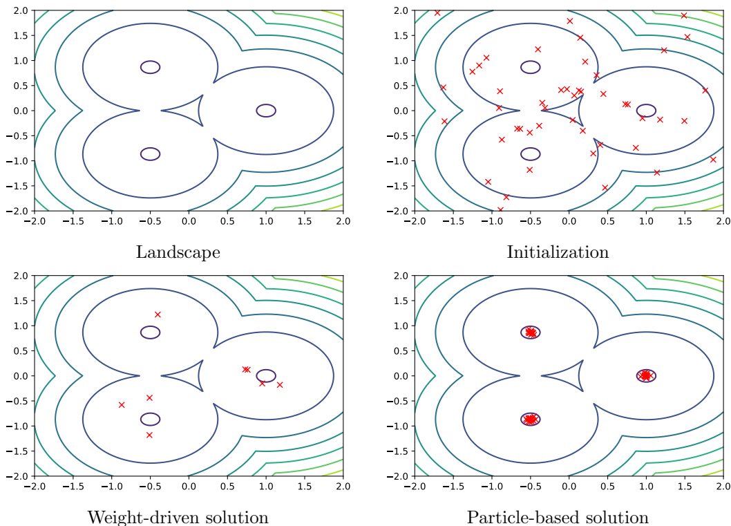
Figure 1: Comparison between weight-driven and particle-based algorithms.
