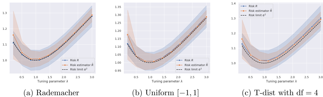
Figure 6: We change the distribution of the design matrix \mathbf{X} to Uniform, Student’s T, and Rademacher distributions with proper normalization so that the variance is 1. Simulation parameter: the noise distribution F_\epsilon = \text{t-dist}(\text{df} = 2) , sample size n = 4000 , feature p = 1200 , scaling parameter \lambda = 1 , 100 repetition.
