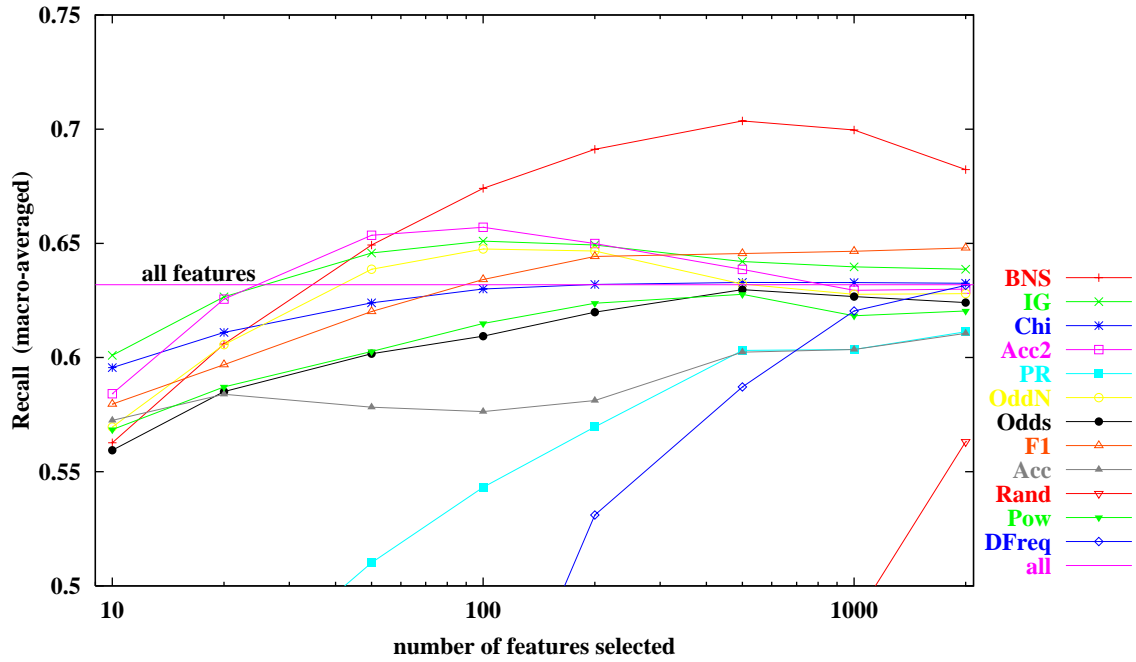
Figure 15. Same as Figure 14, but for recall.
